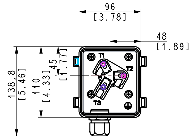
TERMINAL BOX LAYOUT SCALE 1:3
